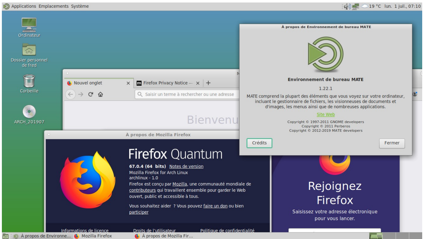
Illustration 16 : Mate Desktop 1.22.1
