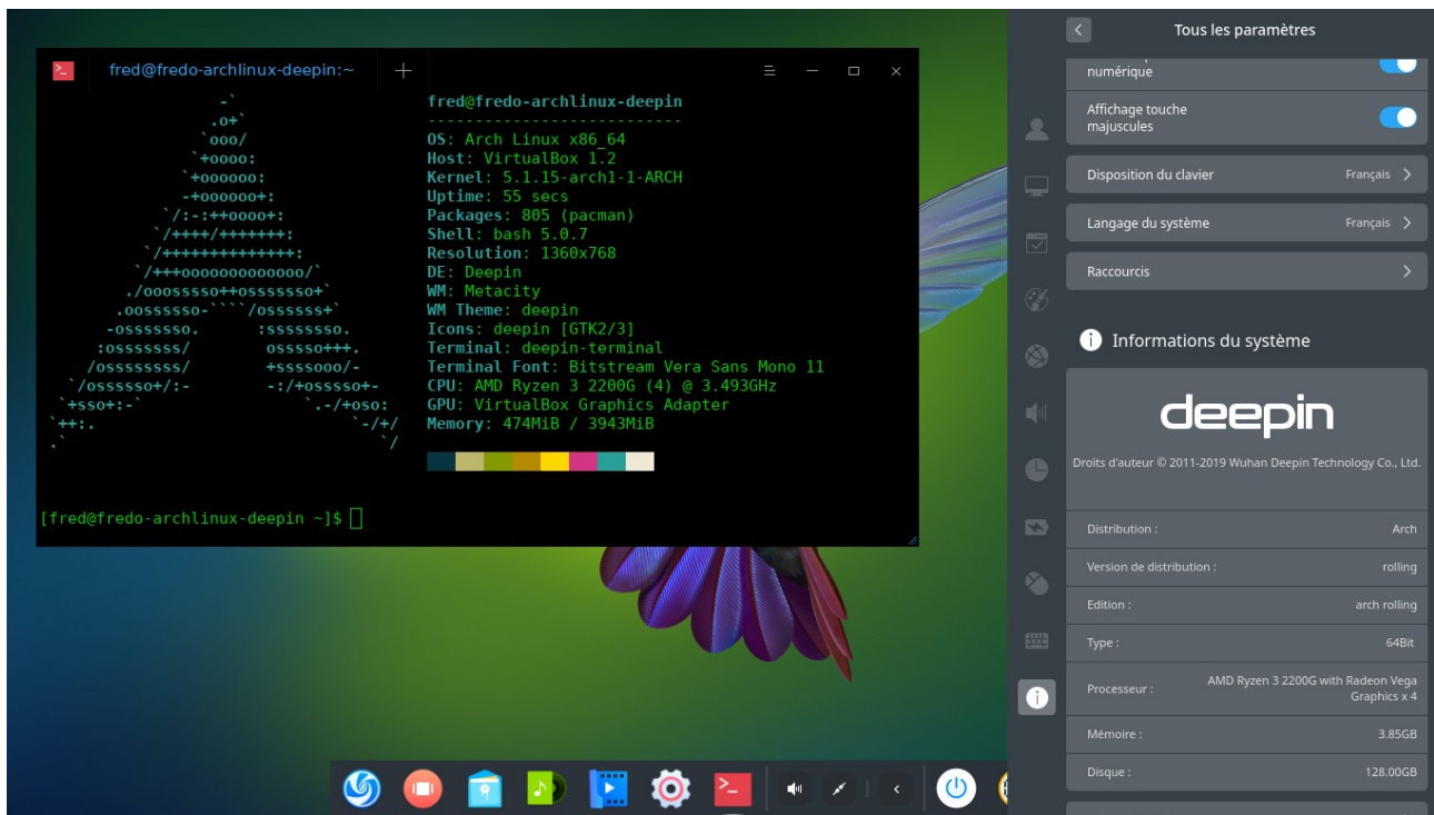
Illustration 17 : Deepin Desktop 15.10.2
